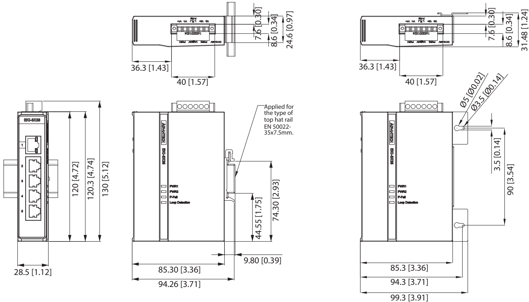
DIN-rail Mounting
