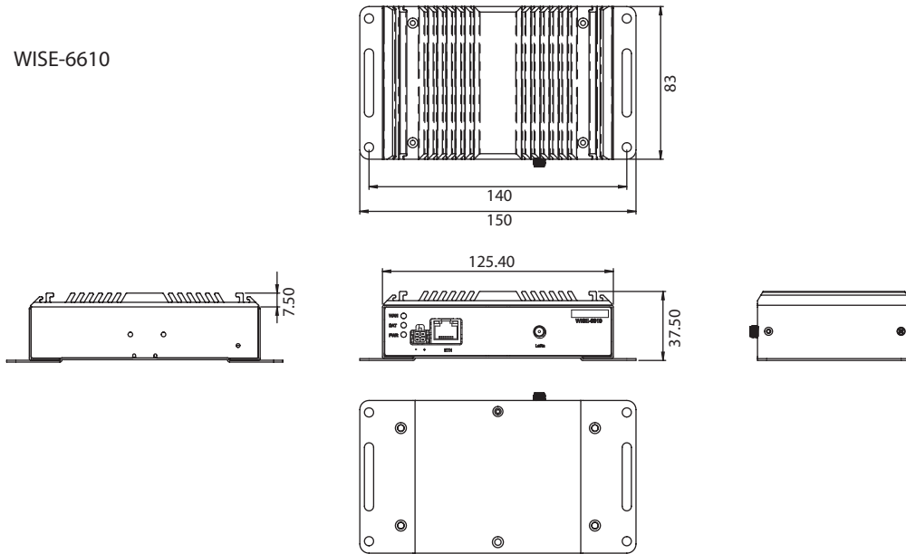
WISE-6610 LTE
