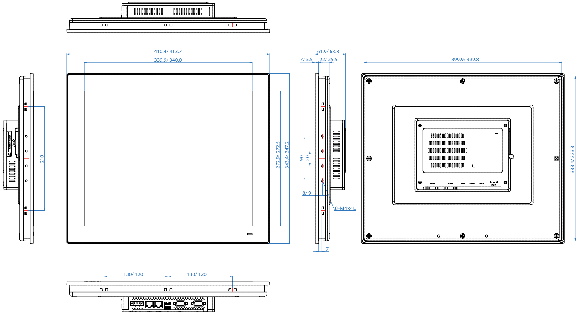
TPC-1751T Panel Cut-out Dimensions: 401.3 x 334.8 mm (15.80" x 13.18")
